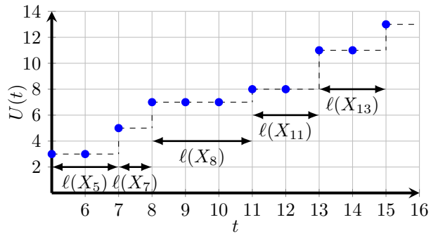
Fig. 2: A sample path of U(t) with U(5) = 3 .
