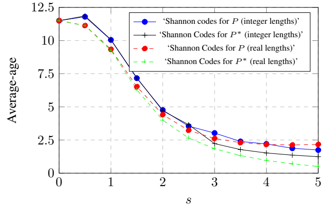
Fig. 3: Comparison of proposed codes and Shannon codes for Zipf( s, 256 ) with varying s . The average age is computed using real-valued lengths as well as lengths rounded-off to integer values.
