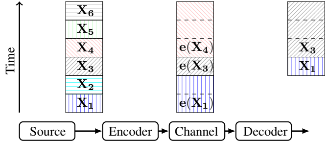
Fig. 1: An example of the proposed memoryless update scheme, where the symbol X_2 is skipped since the channel was busy sending X_1 when it arrived. Furthermore, the decoder retains output X_3 , a symbol which was received within a delay of 1 time unit, for 3 time slots while X_4 was being sent.
