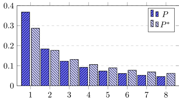
Fig. 4: Pmf for P^* and P for Zipf(1,8).
